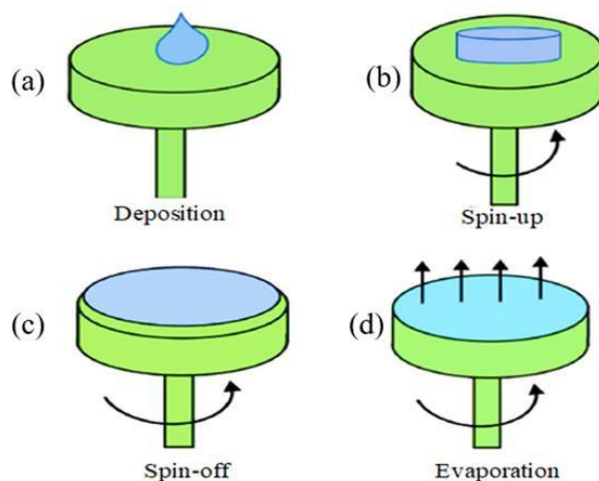
Fig. 1. Four stages of spin coating process
