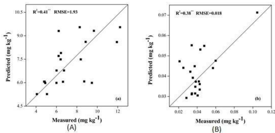
Figure 4. Plot of measured concentrations against the predicted concentration of Cu (a) and Cd (b) of rice leaves using PLSR models.
