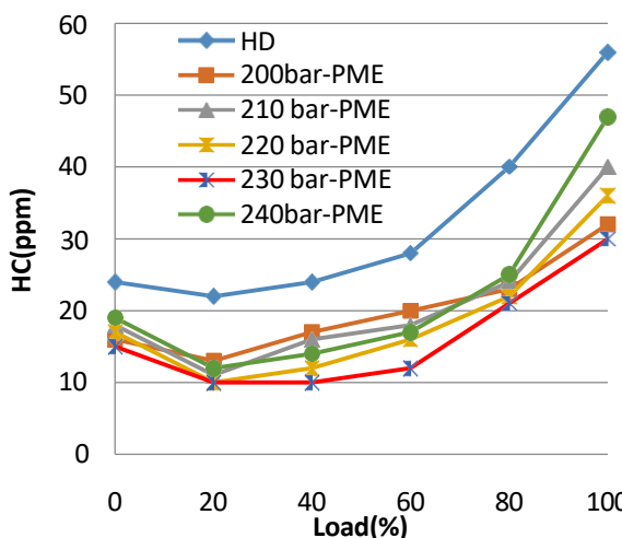
Fig.4.4 HC Variations for different FIPs 26°bTDC
