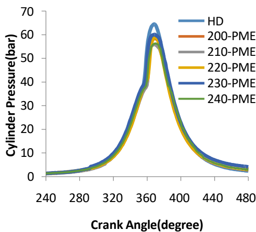
Fig.4.11 CP variation for different FIPs at 80% load
